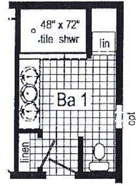
Optional 4'x6' Walk-In Tile Shower
