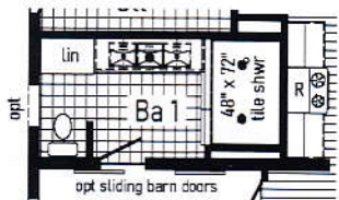
Optional 4'x6' Walk-In Tile Shower (omits broom closet)
